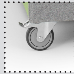
Castors with treads made of thermoplastic polyurethane, with an anti-ling cover. Two wheels with the „stop-fix” turn head block.
